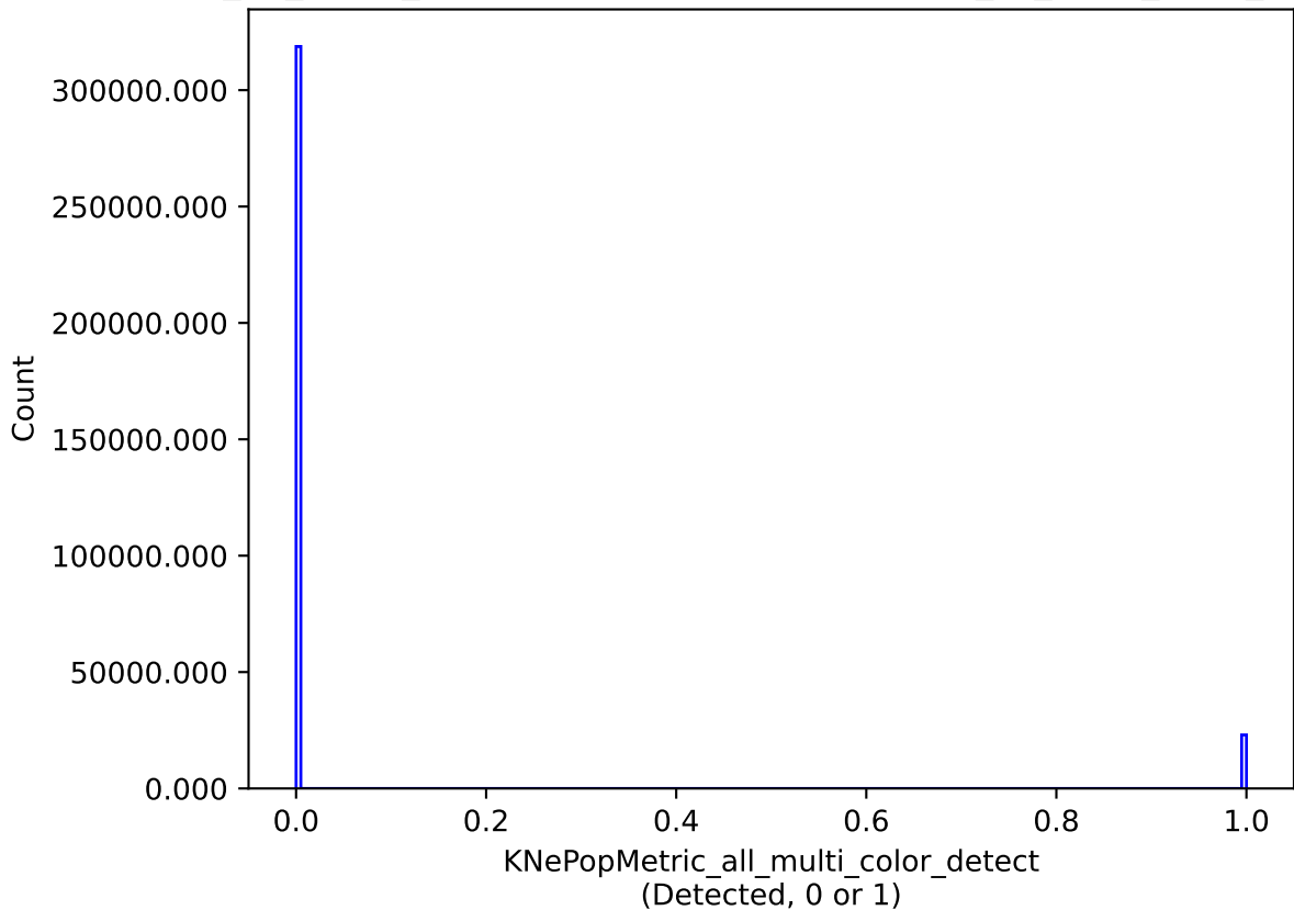
too_10_1v3.4_10yrs all models: KNePopMetric_all_multi_color_detect
