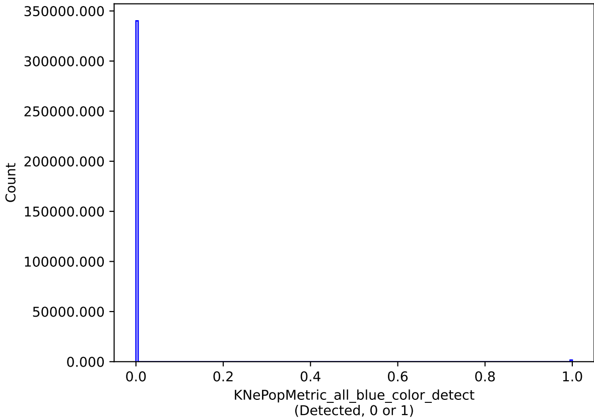
too_10_1v3.4_10yrs all models: KNePopMetric_all_blue_color_detect
