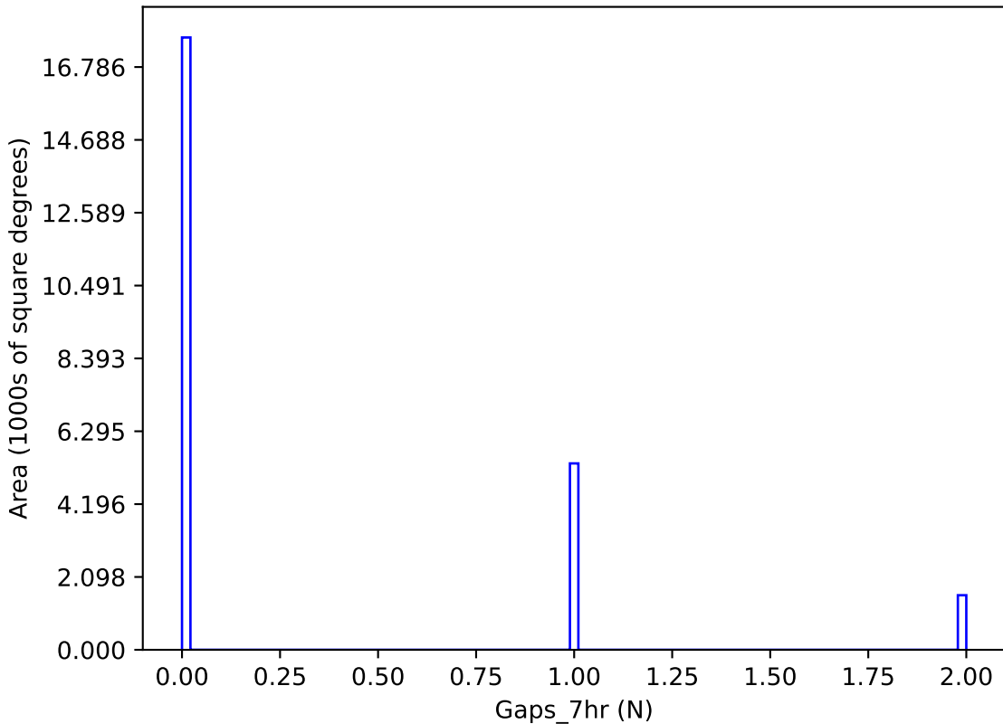
too_10_1v3.4_10yrs y band: Gaps_7hr
