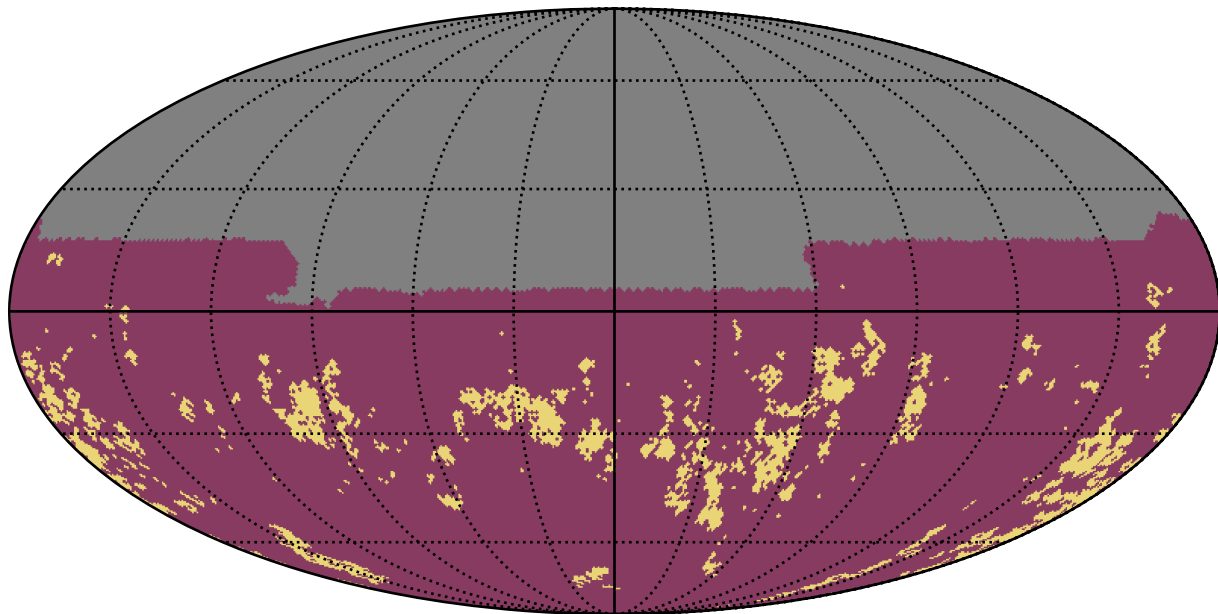
too_10_1v3.4_10yrs u band: Gaps_7hr
