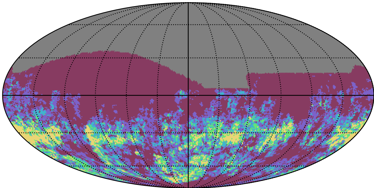
too_10_1v3.4_10yrs r band: Gaps_7hr
