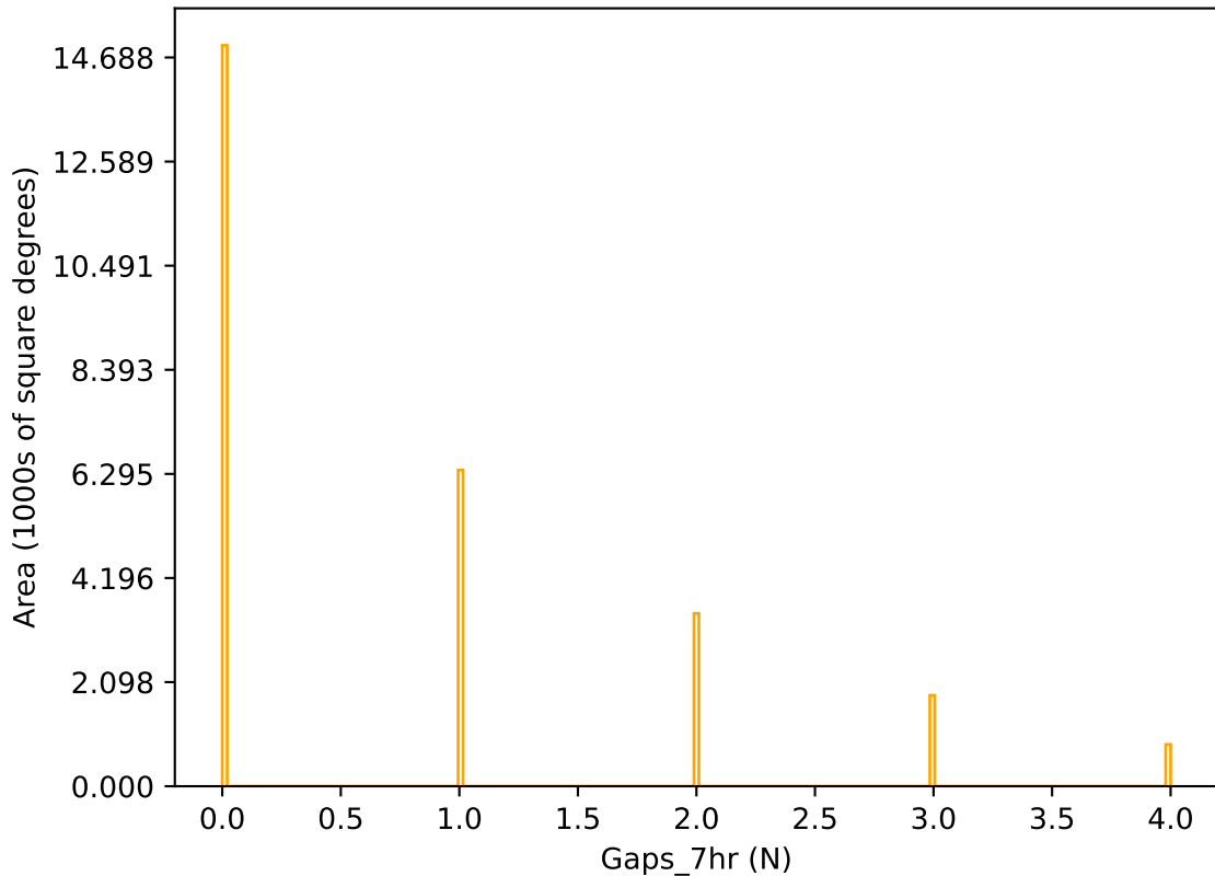
too_10_1v3.4_10yrs r band: Gaps_7hr
