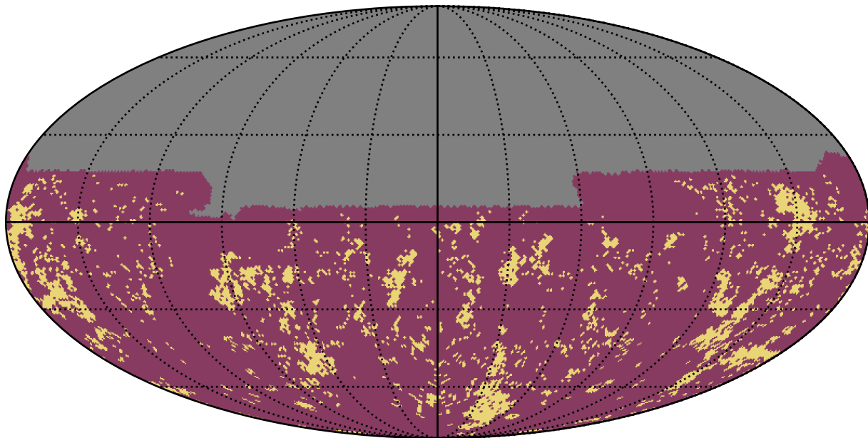
too_10_1v3.4_10yrs u band: Gaps_3hr
