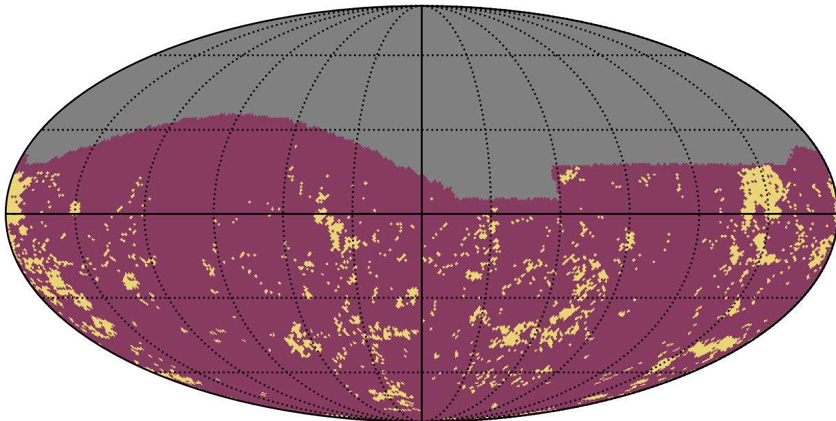
too_10_1v3.4_10yrs g band: Gaps_3hr
