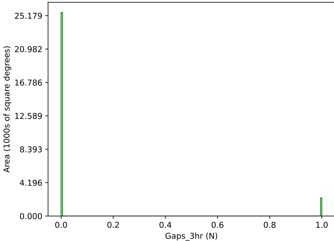
too_10_1v3.4_10yrs g band: Gaps_3hr
