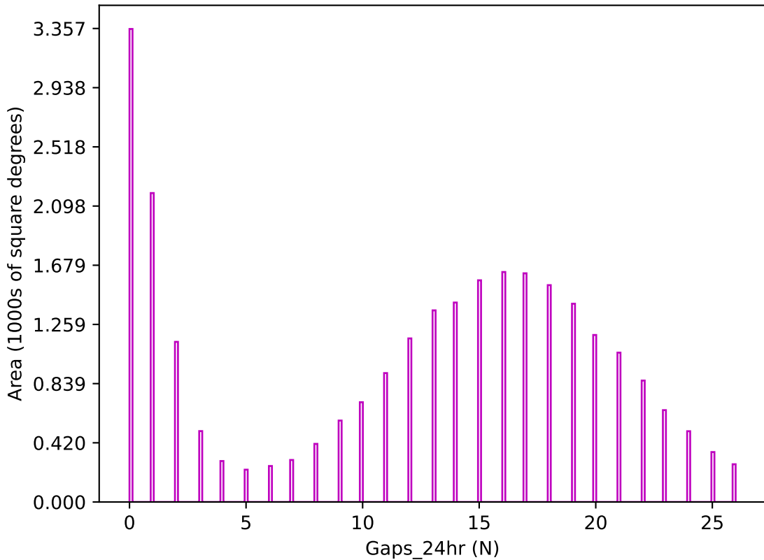
too_10_1v3.4_10yrs z band: Gaps_24hr
