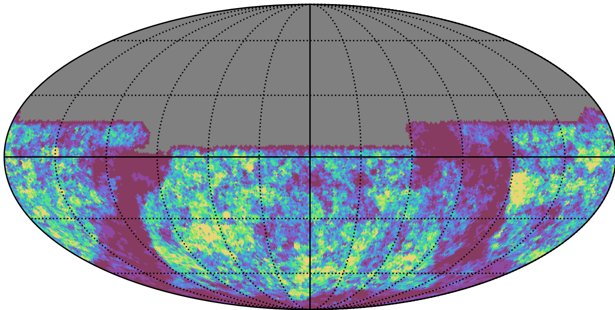
too_10_1v3.4_10yrs u band: Gaps_24hr
