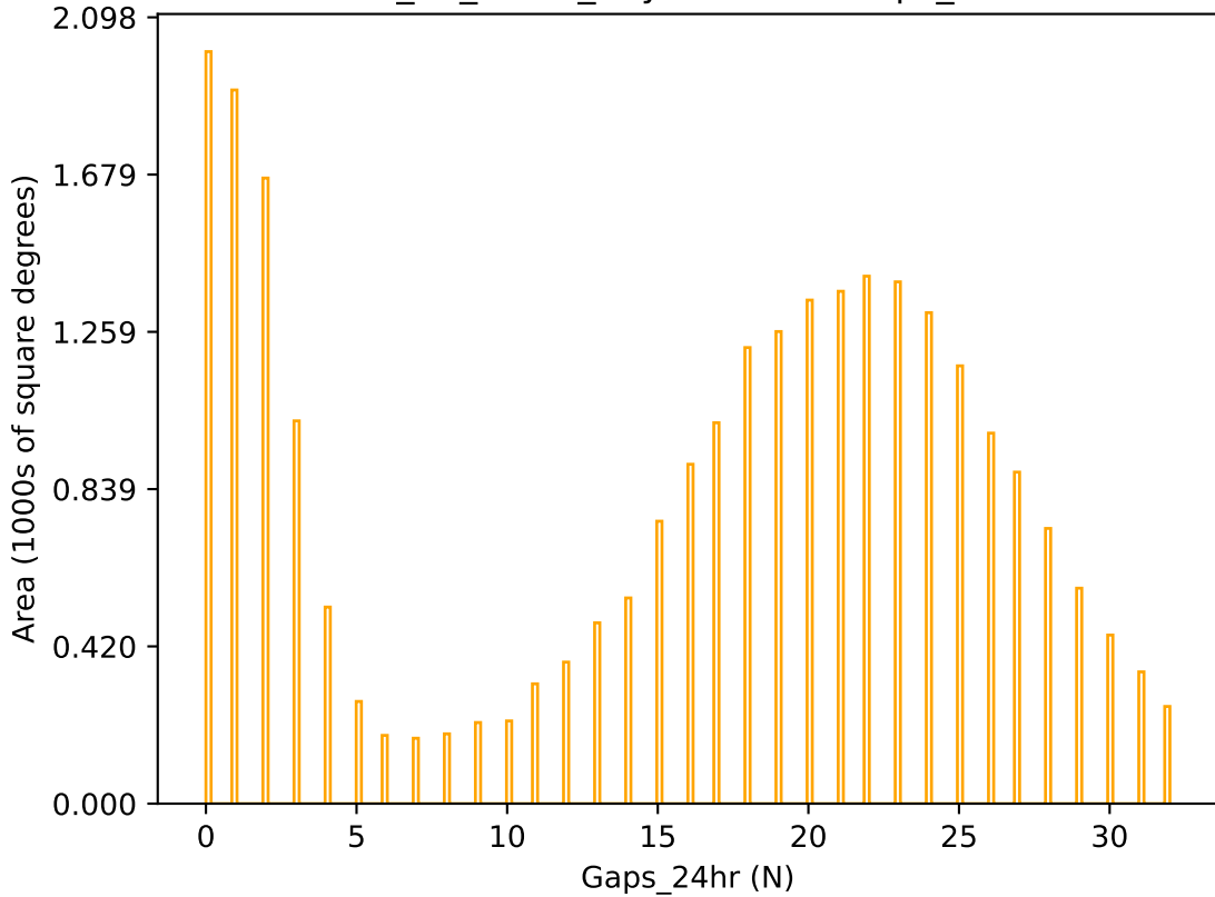
too_10_1v3.4_10yrs r band: Gaps_24hr
