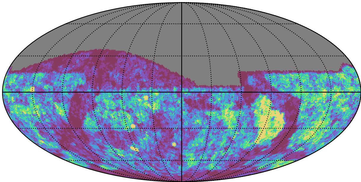
too_10_1v3.4_10yrs g band: Gaps_24hr
