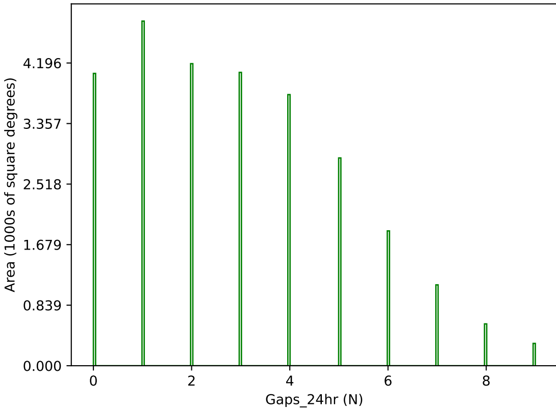
too_10_1v3.4_10yrs g band: Gaps_24hr
