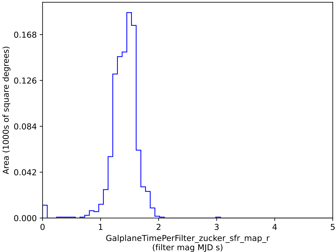
too_10_1v3.4_10yrs : GalplaneTimePerFilter_zucker_sfr_map_r
