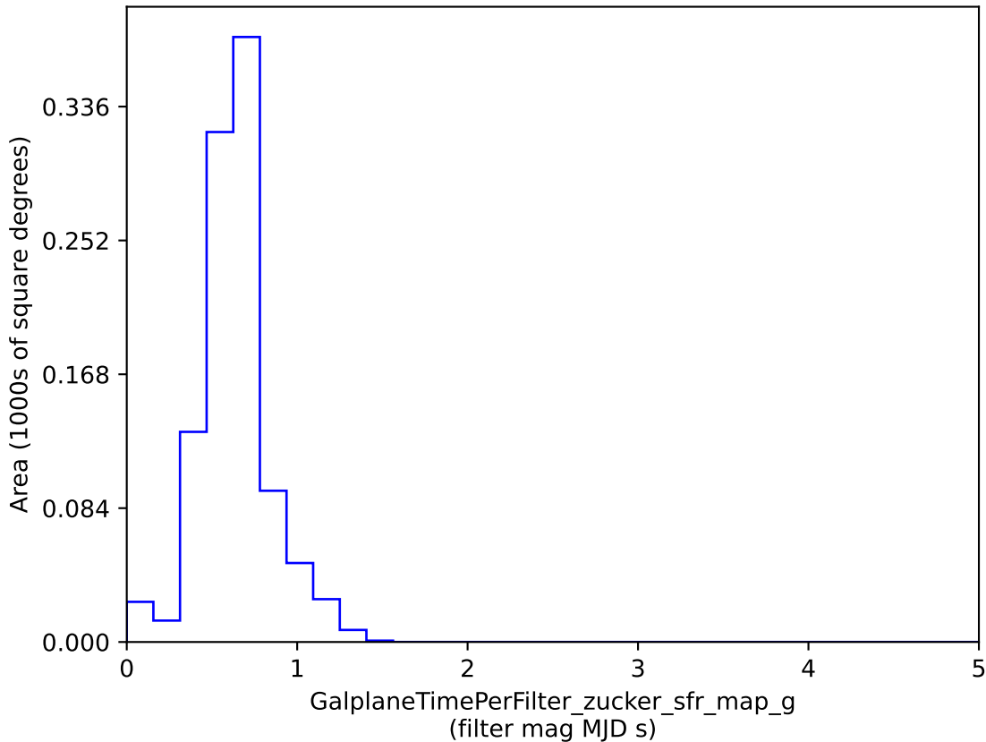
too_10_1v3.4_10yrs : GalplaneTimePerFilter_zucker_sfr_map_g
