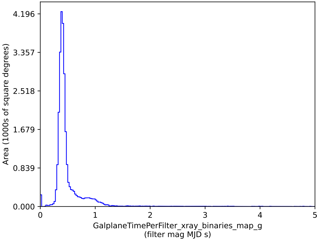
too_10_1v3.4_10yrs : GalplaneTimePerFilter_xray_binaries_map_g
