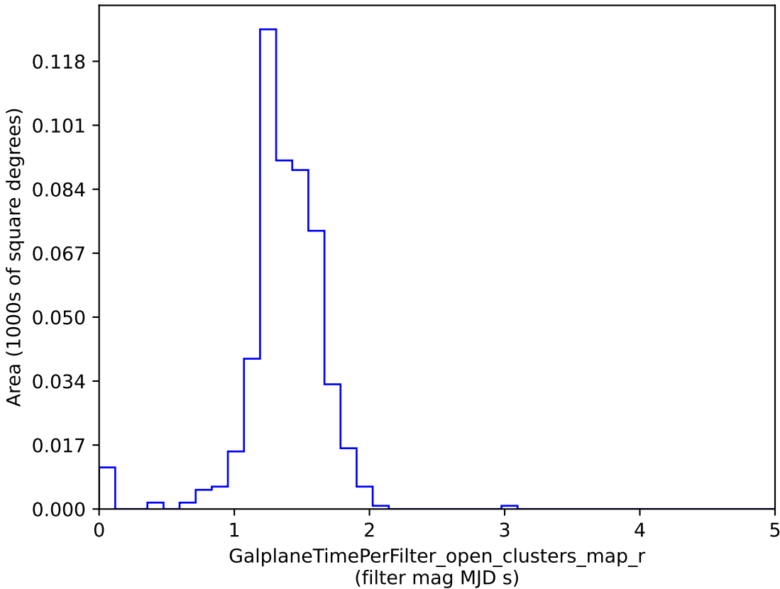
too_10_1v3.4_10yrs : GalplaneTimePerFilter_open_clusters_map_r
