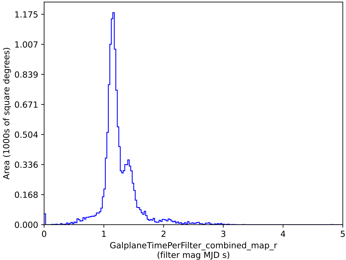
too_10_1v3.4_10yrs : GalplaneTimePerFilter_combined_map_r
