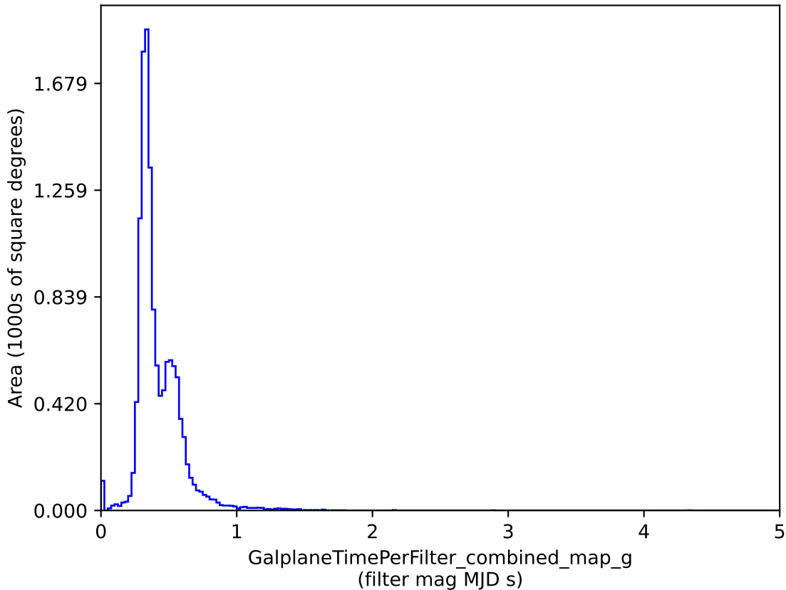
too_10_1v3.4_10yrs : GalplaneTimePerFilter_combined_map_g
