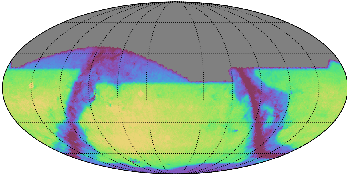
too_10_1v3.4_10yrs z: GalaxyCountsMetricExtended
