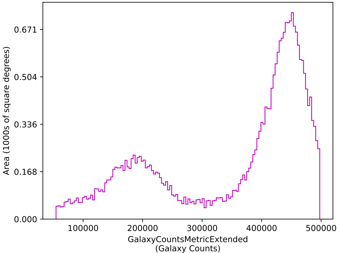
too_10_1v3.4_10yrs z: GalaxyCountsMetricExtended
