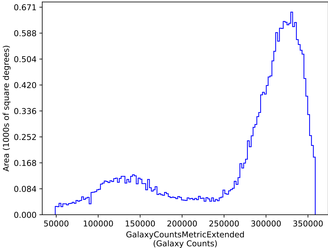
too_10_1v3.4_10yrs y: GalaxyCountsMetricExtended
