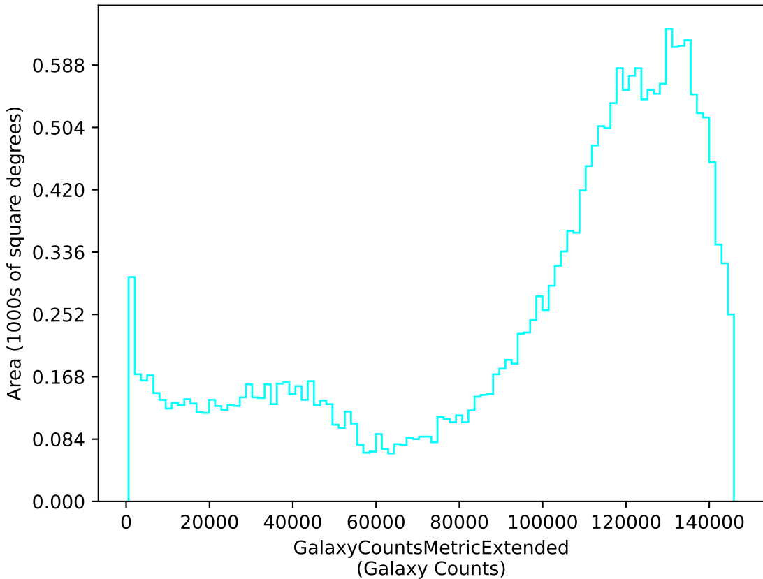
too_10_1v3.4_10yrs u: GalaxyCountsMetricExtended
