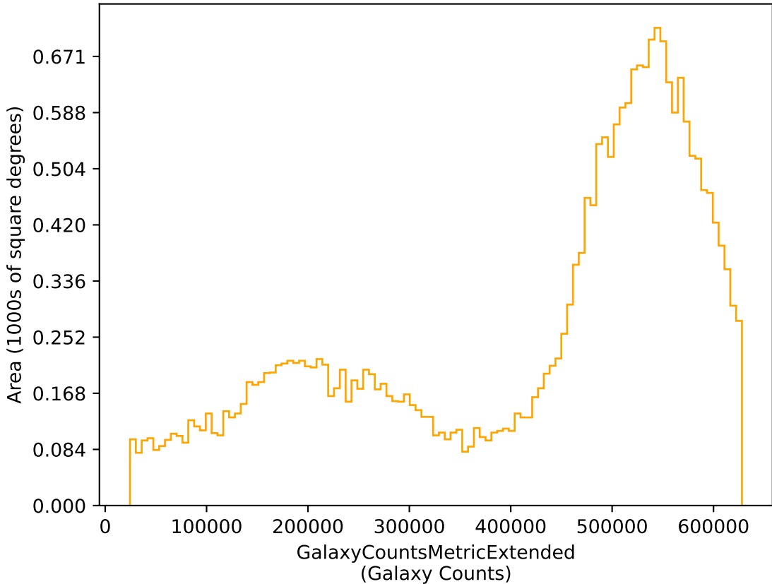
too_10_1v3.4_10yrs r: GalaxyCountsMetricExtended
