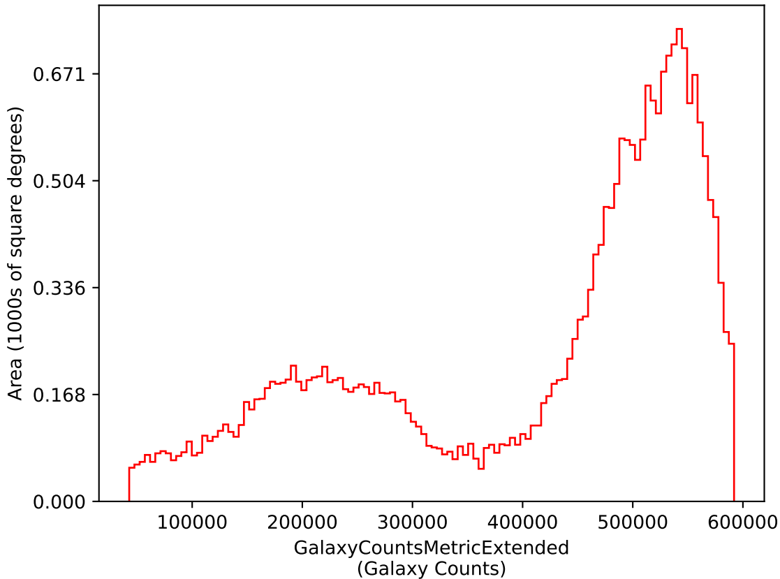
too_10_1v3.4_10yrs i: GalaxyCountsMetricExtended
