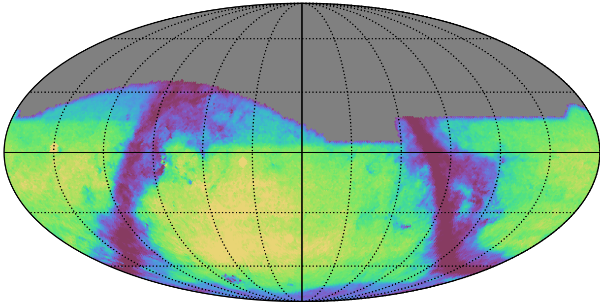
too_10_1v3.4_10yrs g: GalaxyCountsMetricExtended
