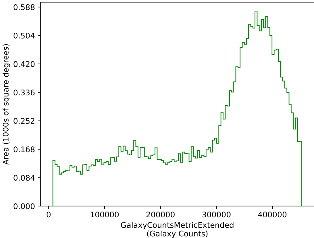
too_10_1v3.4_10yrs g: GalaxyCountsMetricExtended
