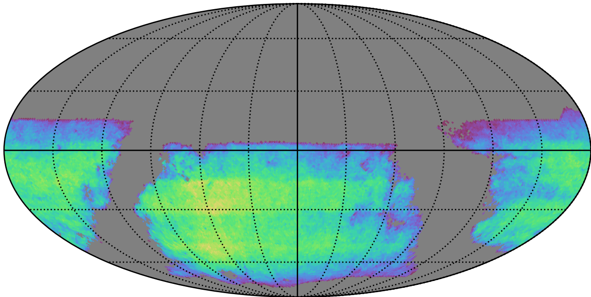
too_10_1v3.4_10yrs i band non-DD year 9: ExgalM5WithCuts
