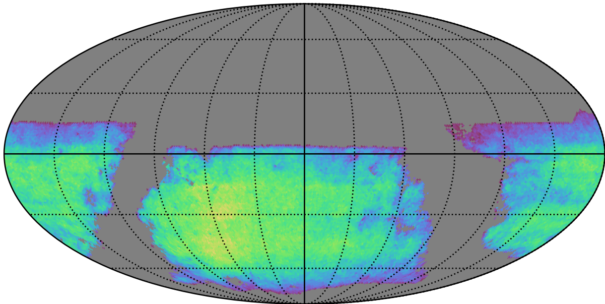
too_10_1v3.4_10yrs i band non-DD year 8: ExgalM5WithCuts
