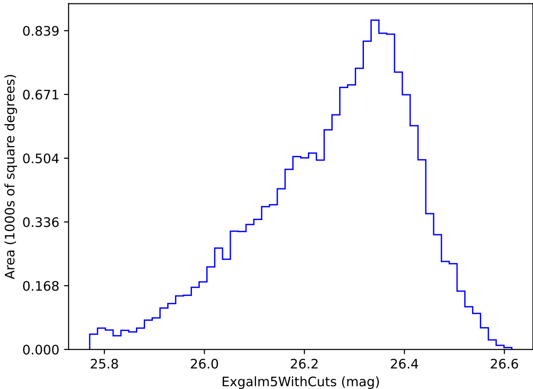
too_10_1v3.4_10yrs i band non-DD year 8: ExgalM5WithCuts
