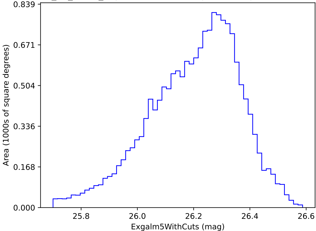
too_10_1v3.4_10yrs i band non-DD year 7: ExgalM5WithCuts
