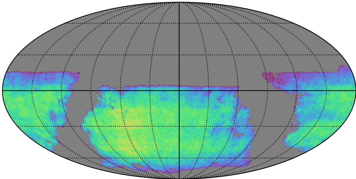
too_10_1v3.4_10yrs i band non-DD year 6: ExgalM5WithCuts
