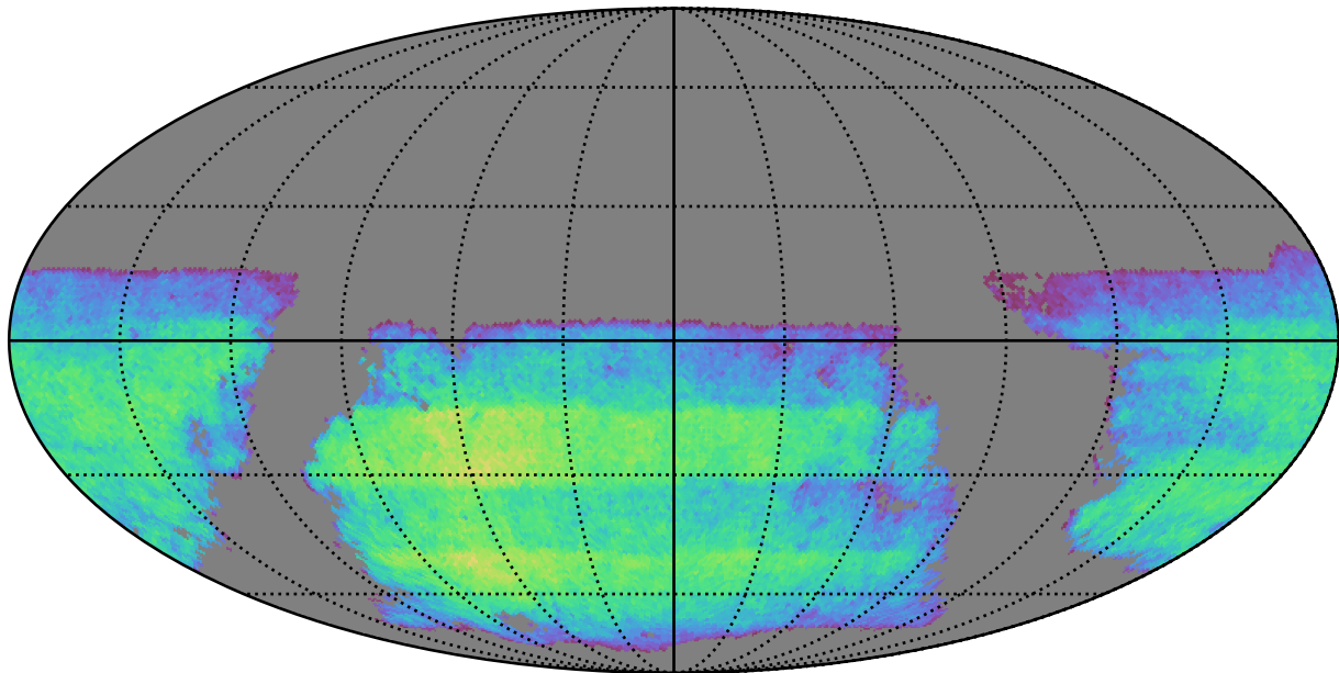
too_10_1v3.4_10yrs i band non-DD year 5: ExgalM5WithCuts
