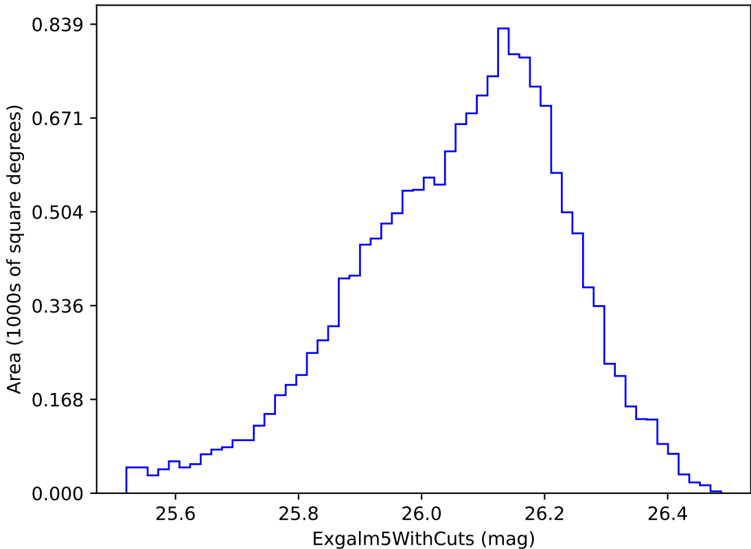
too_10_1v3.4_10yrs i band non-DD year 5: ExgalM5WithCuts
