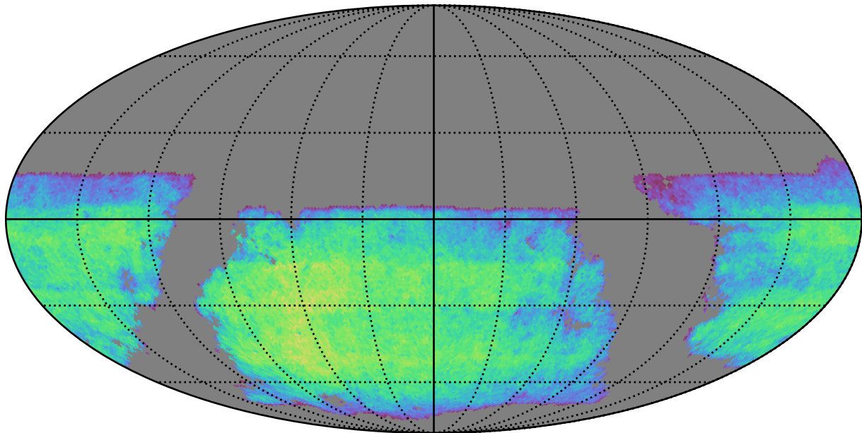
too_10_1v3.4_10yrs i band non-DD year 4: ExgalM5WithCuts
