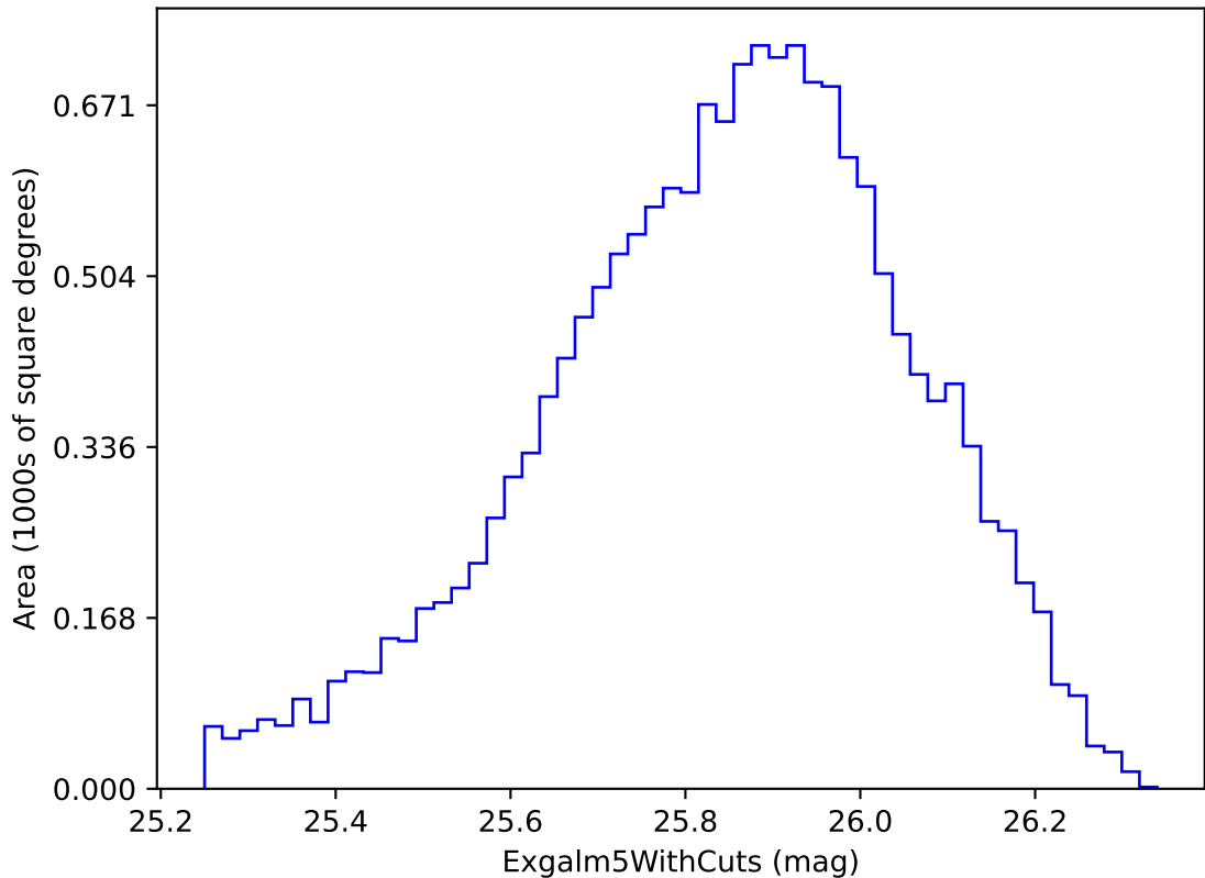
too_10_1v3.4_10yrs i band non-DD year 3: ExgalM5WithCuts
