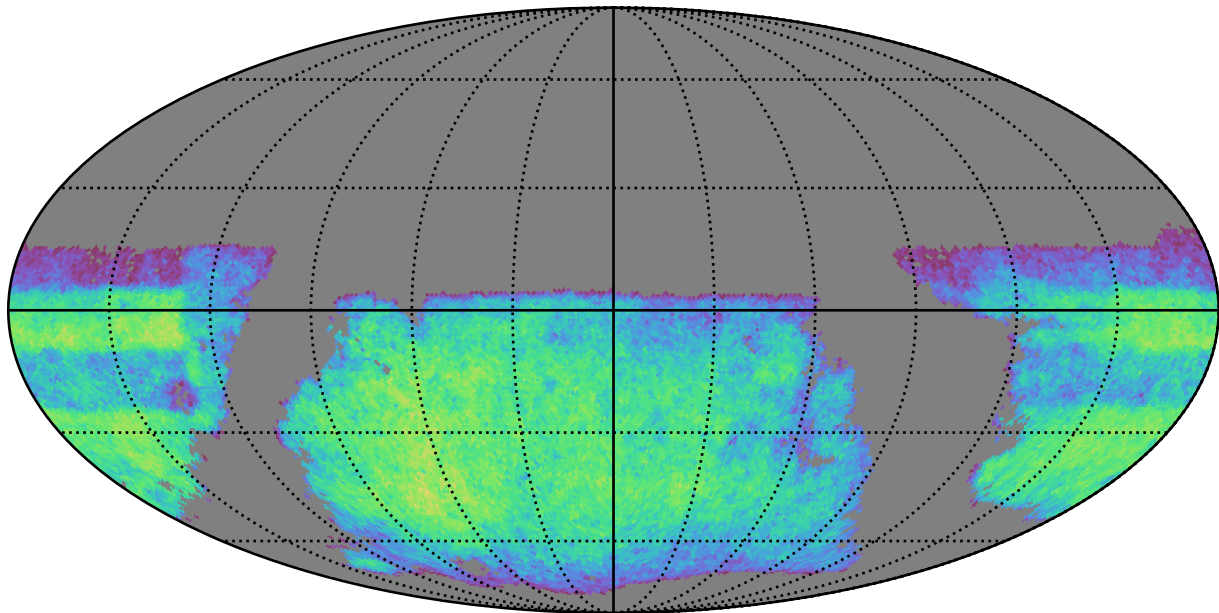
too_10_1v3.4_10yrs i band non-DD year 2: ExgalM5WithCuts
