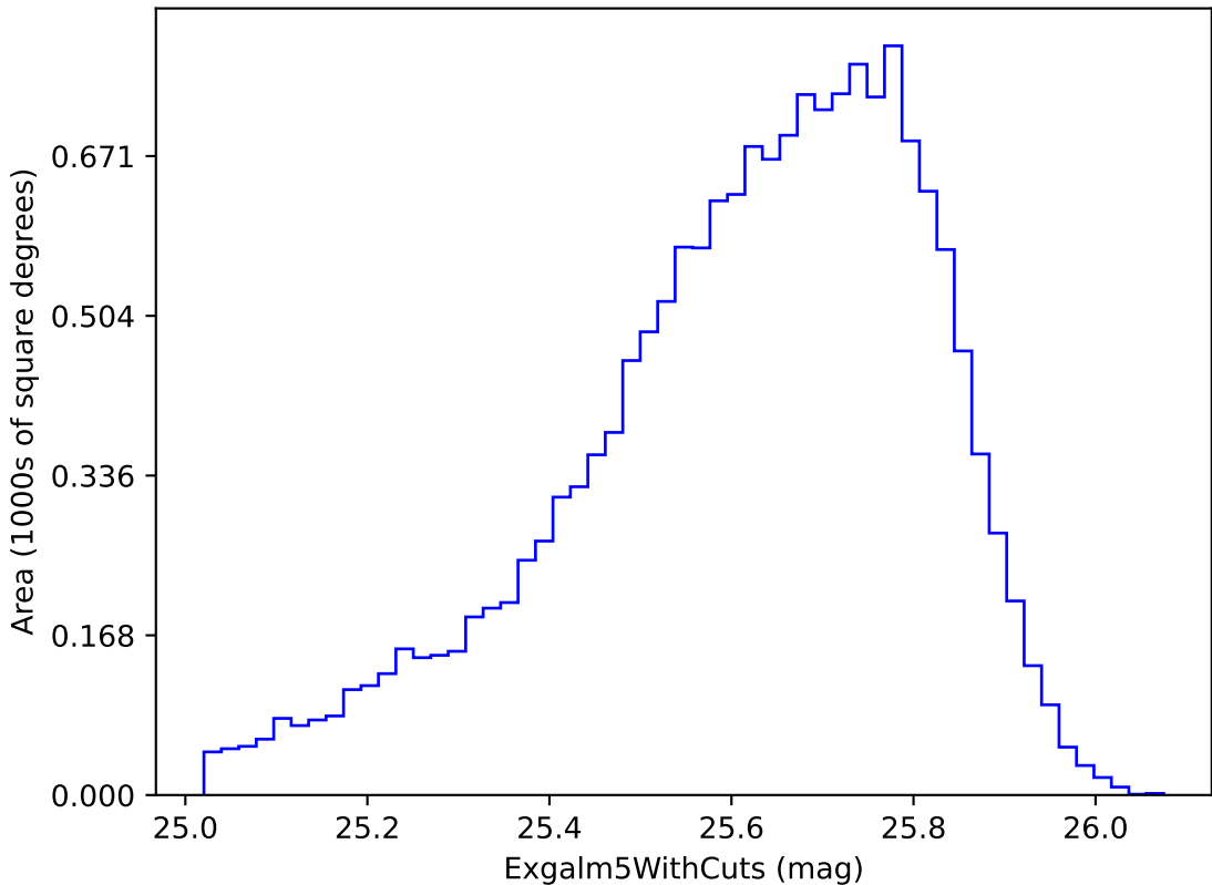
too_10_1v3.4_10yrs i band non-DD year 2: ExgalM5WithCuts
