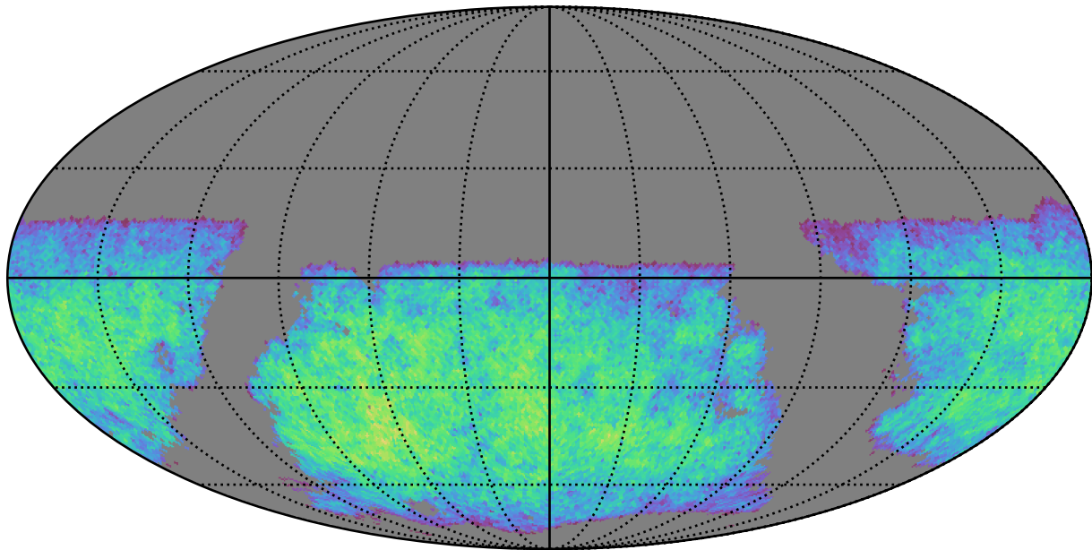
too_10_1v3.4_10yrs i band non-DD year 1: ExgalM5WithCuts
