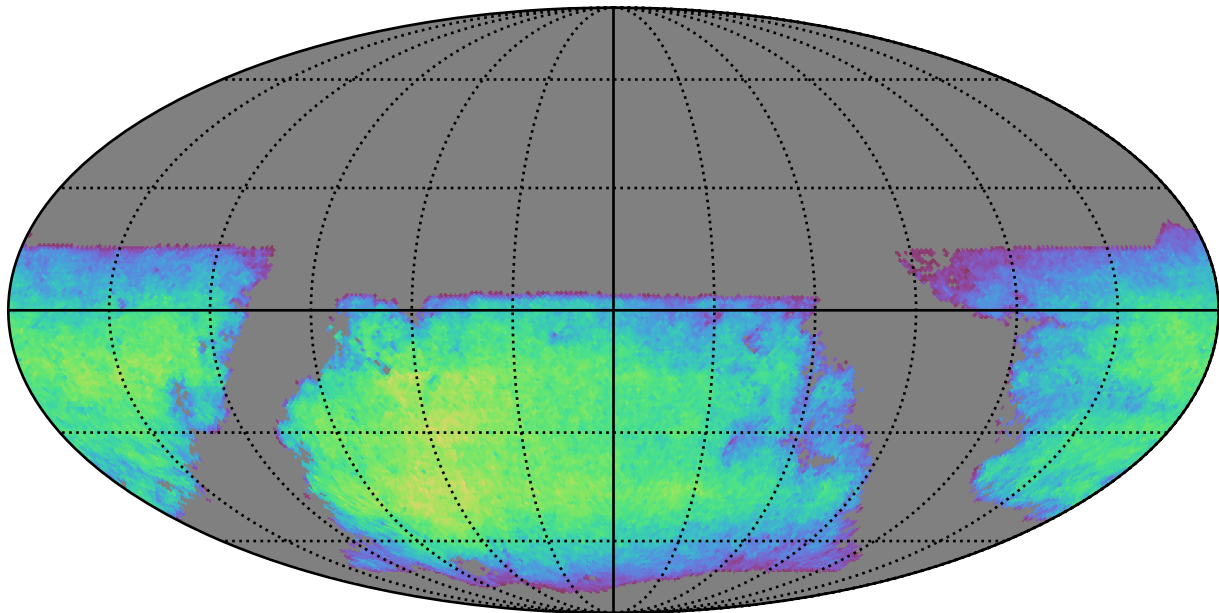
too_10_1v3.4_10yrs i band non-DD year 10: ExgalM5WithCuts
