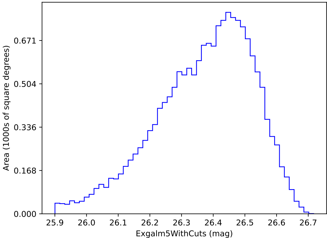
too_10_1v3.4_10yrs i band non-DD year 10: ExgalM5WithCuts
