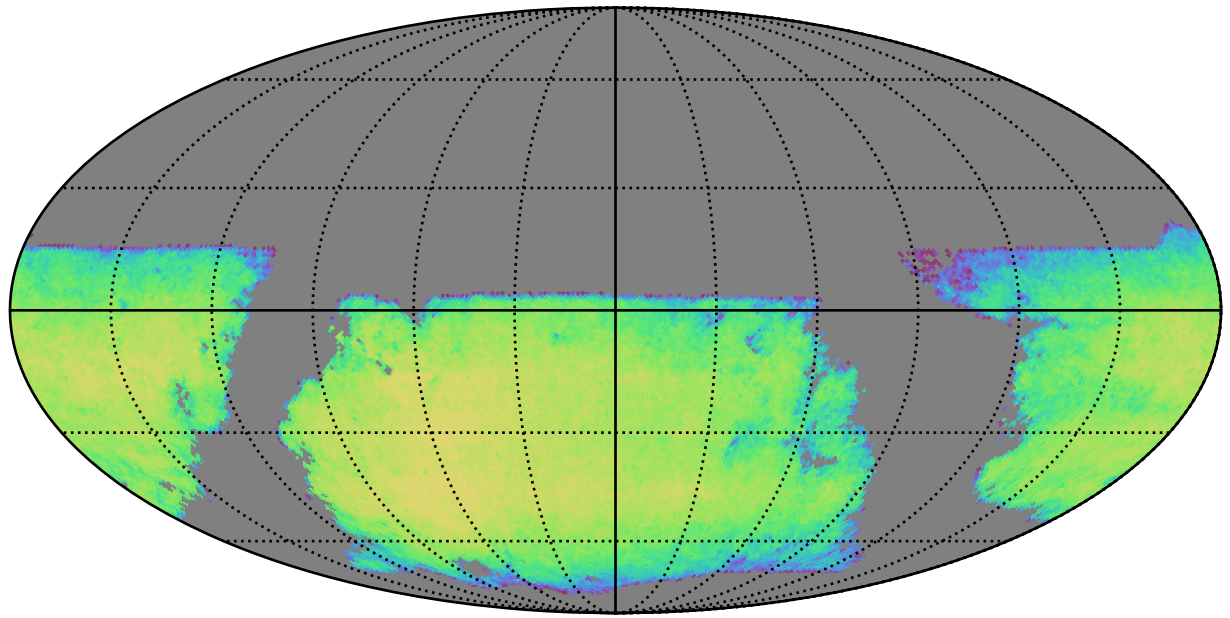
too_10_1v3.4_10yrs i band galaxies non-DD: DepthLimitedNumGalaxiesMetric
