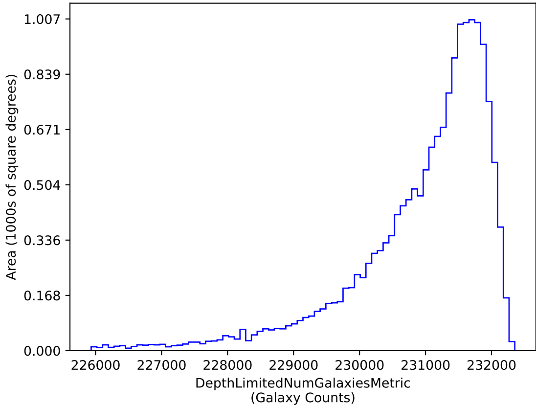
too_10_1v3.4_10yrs i band galaxies non-DD: DepthLimitedNumGalaxiesMetric
