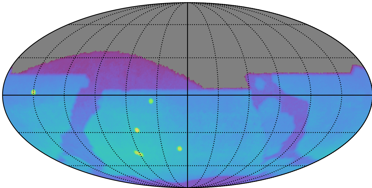
too_10_1v3.4_10yrs : Brown Dwarf, L7
