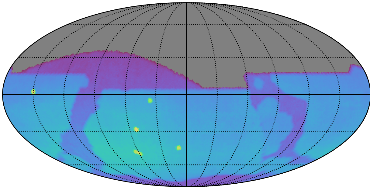
too_10_1v3.4_10yrs : Brown Dwarf, L4
