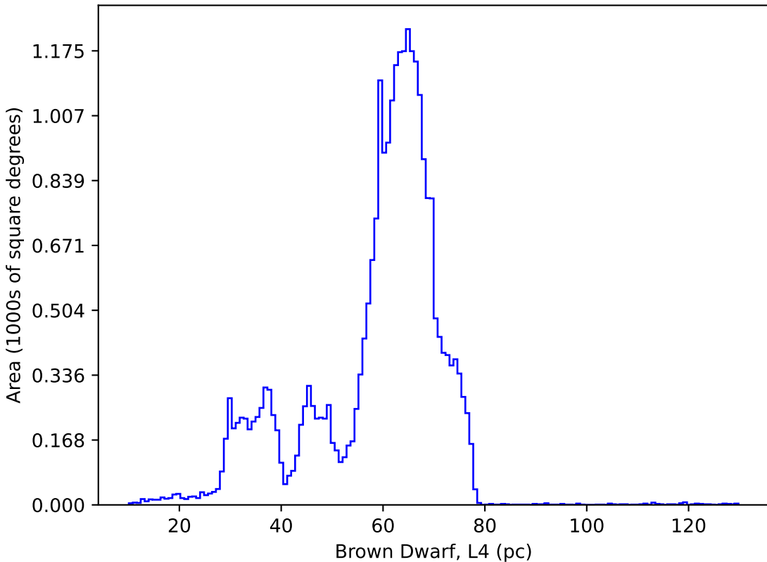
too_10_1v3.4_10yrs : Brown Dwarf, L4
