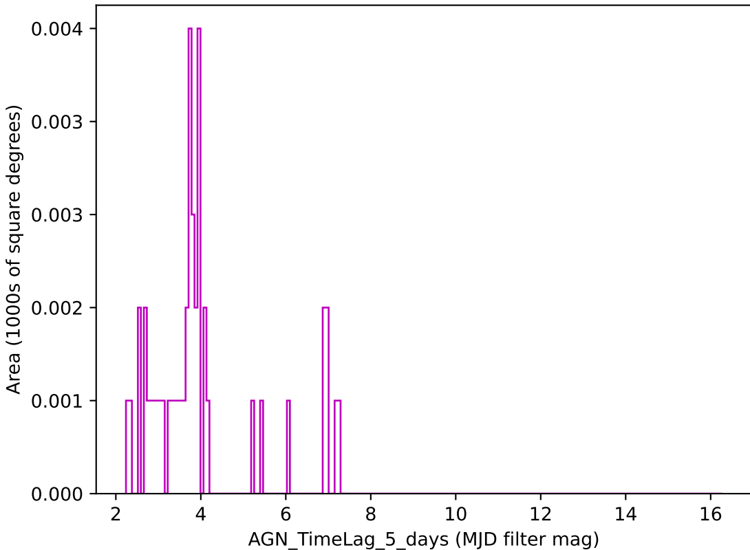
too_10_1v3.4_10yrs z band: AGN_TimeLag_5_days
