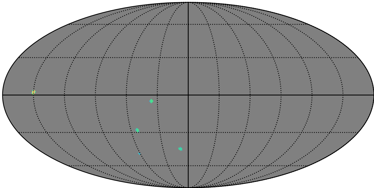
too_10_1v3.4_10yrs r band: AGN_TimeLag_5_days
