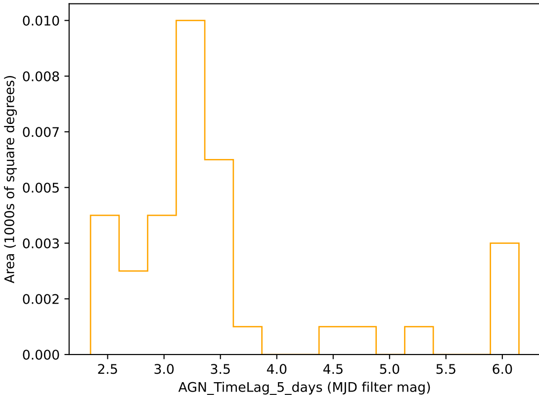
too_10_1v3.4_10yrs r band: AGN_TimeLag_5_days
